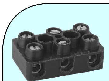
Terminal Block suitable for New 3 Pin Connector
