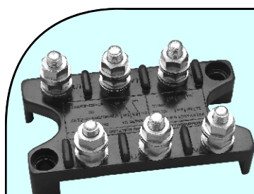
Terminal Block suitable for Kirloskar 40-60 HP
