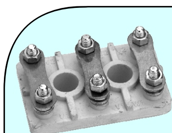
Terminal Block suitable for Siemens / Hindustan GN-100-132 frame
