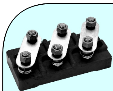
Terminal Block 175 x 82 (M 12)
