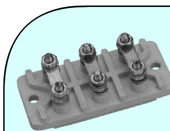
Terminal Block suitable for Siemens / Hindustan GN-63-90 Frame
