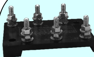
Terminal Block suitable for Kirloskar 100 HP
